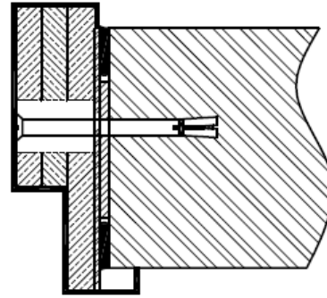
Slide in Steel frame with Dynabolt fixings at typically 400mm centres (up to 2 hours)
