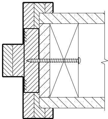
MS tube or saddle bracket
