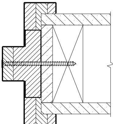
Countersunk screw
