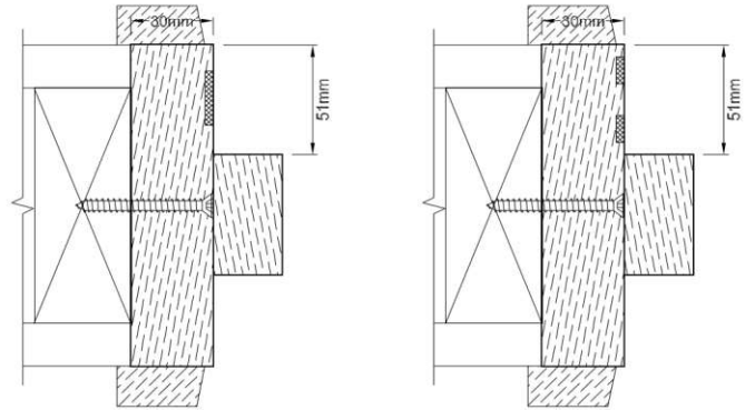
Typical frame profile
