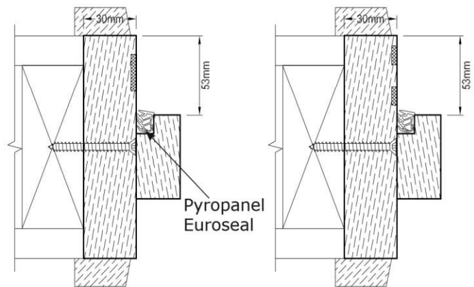
Euroseal frame profile
