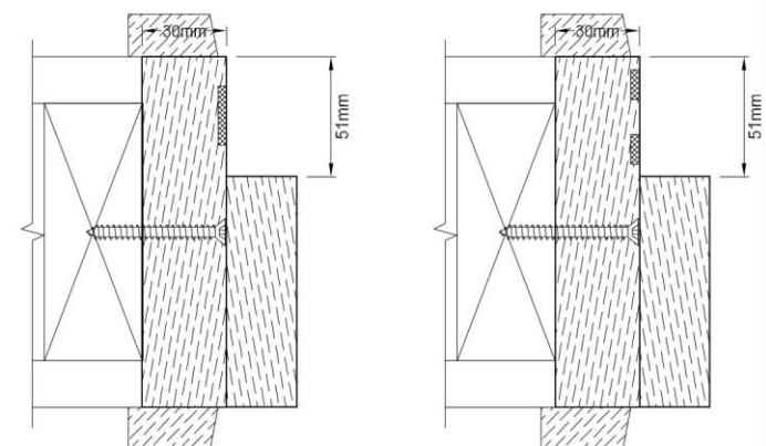
Alternative frame profile (Single rebate)
