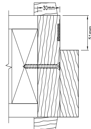
Alternative frame profile (Single rebate)
