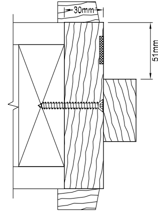
Typical frame profile
