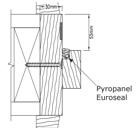
Euroseal frame profile
