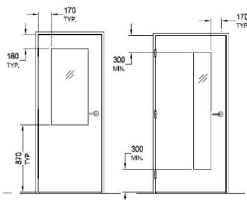
Half-lite
